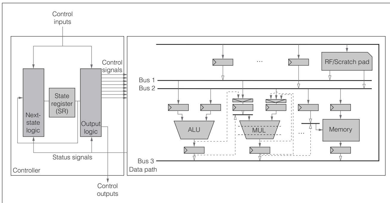
Figure 2. Typical architecture.
